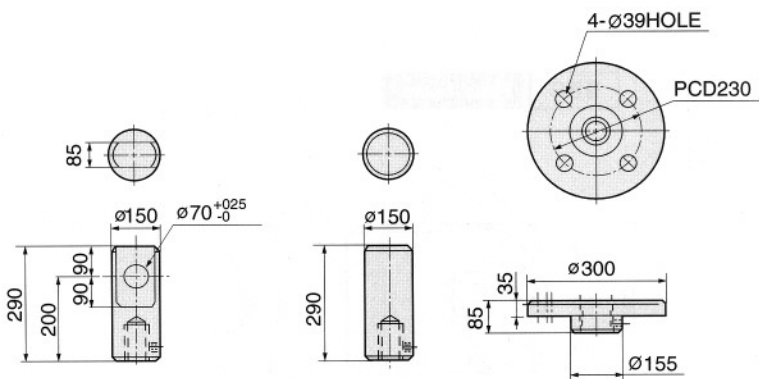
Dimension of Screw Nut
