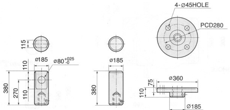
Dimension of Screw Nut
